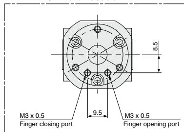
MDHR2-10E Port Location
