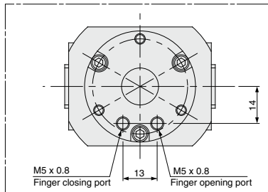
MDHR2-20E Port Location
