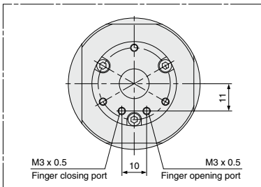
MDHR3-15E Port Location
