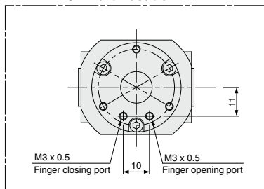
MDHR2-15E Port Location
