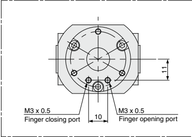
MHR2-15E Port Location
