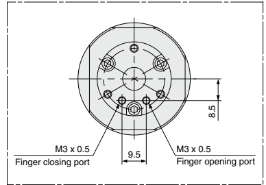
MDHR3-10E Port Location
