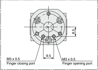
MHR2-10E Port Location
