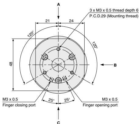
MDHR3-15E Port Location
