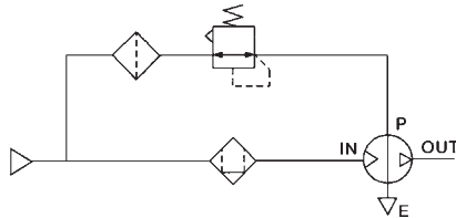
Pilot regulator
