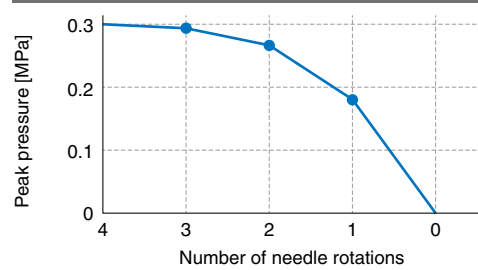
Peak pressure and the number of needle rotations (Supply pressure: 0.5 MPa)
