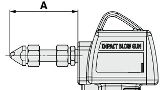
Long nozzle with a silencer
