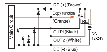
KP43 □ - 02 - □ 2 NPN + Copy Function
